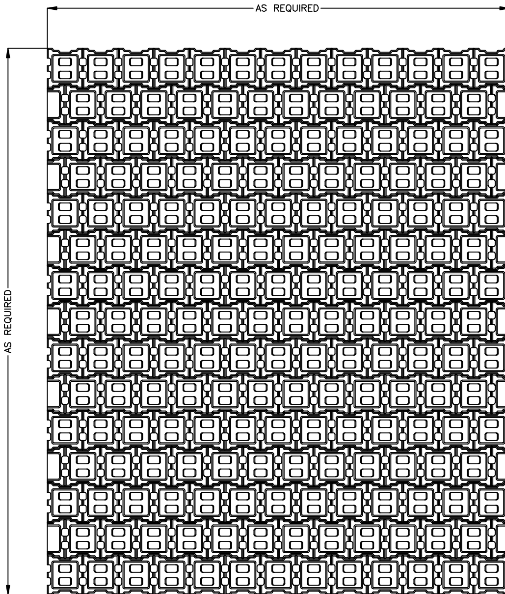
PLAN ARMORFLEX PLACEMENT NOT TO SCALE
