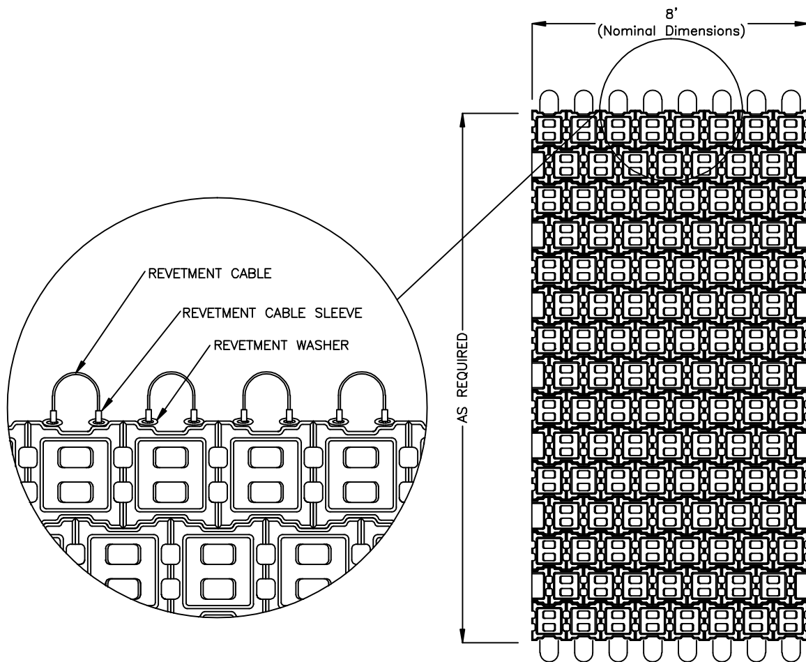
TYPICAL ARMORFLEX MAT NOT TO SCALE
