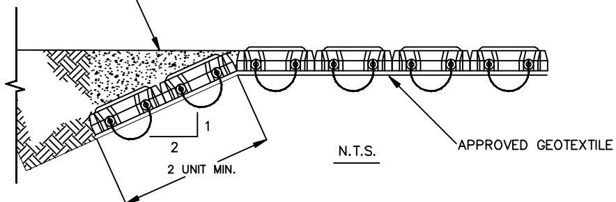
TYPICAL ARMORFLEX MAT NOT TO SCALE
