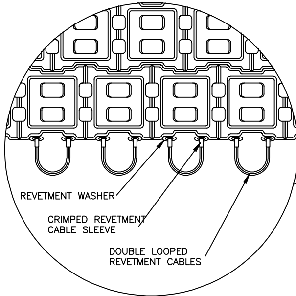
DOUBLE LOOP END
