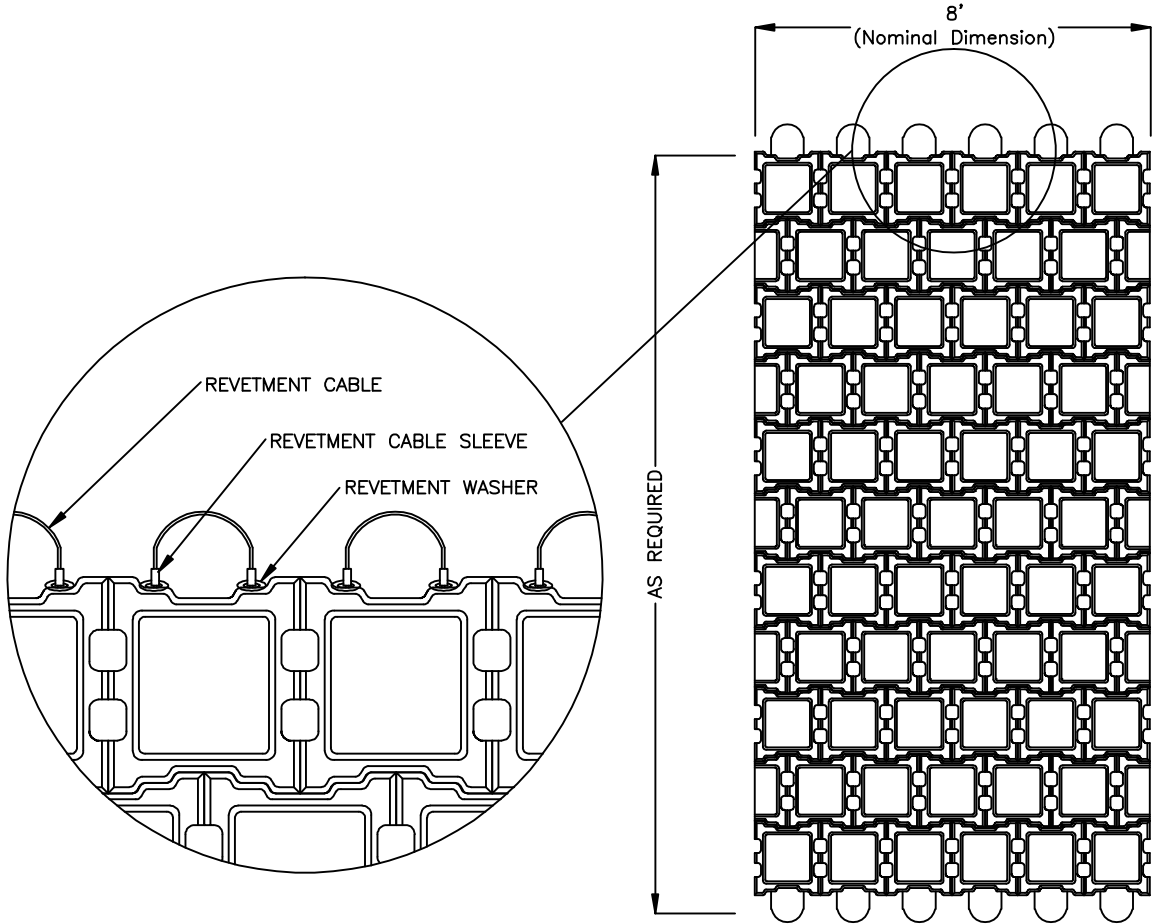
PLAN
