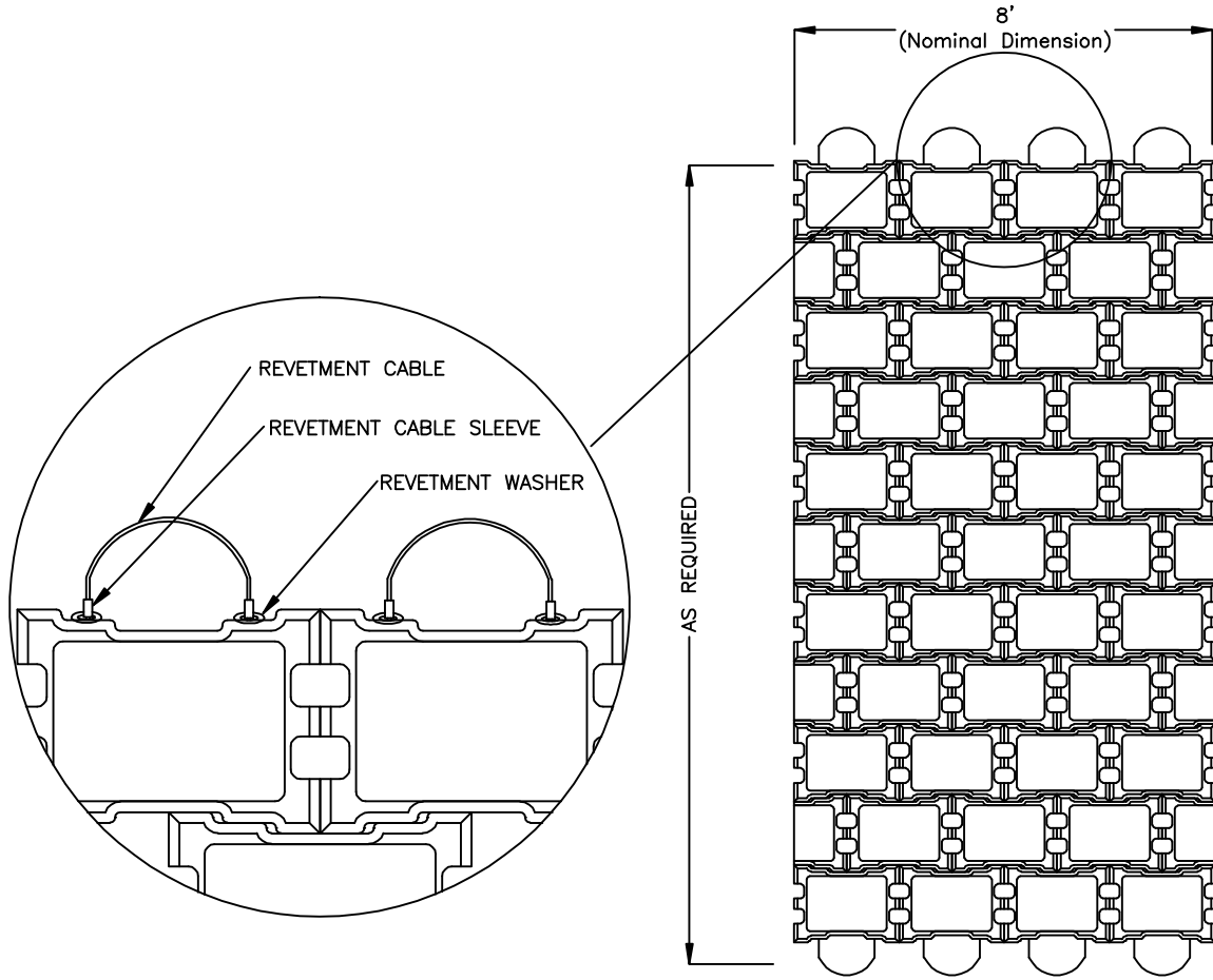
PLAN
